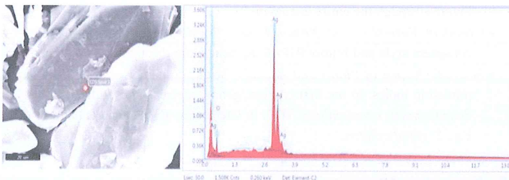
Figure 2.1.3: EDS spectra of silver vein graphite composite
